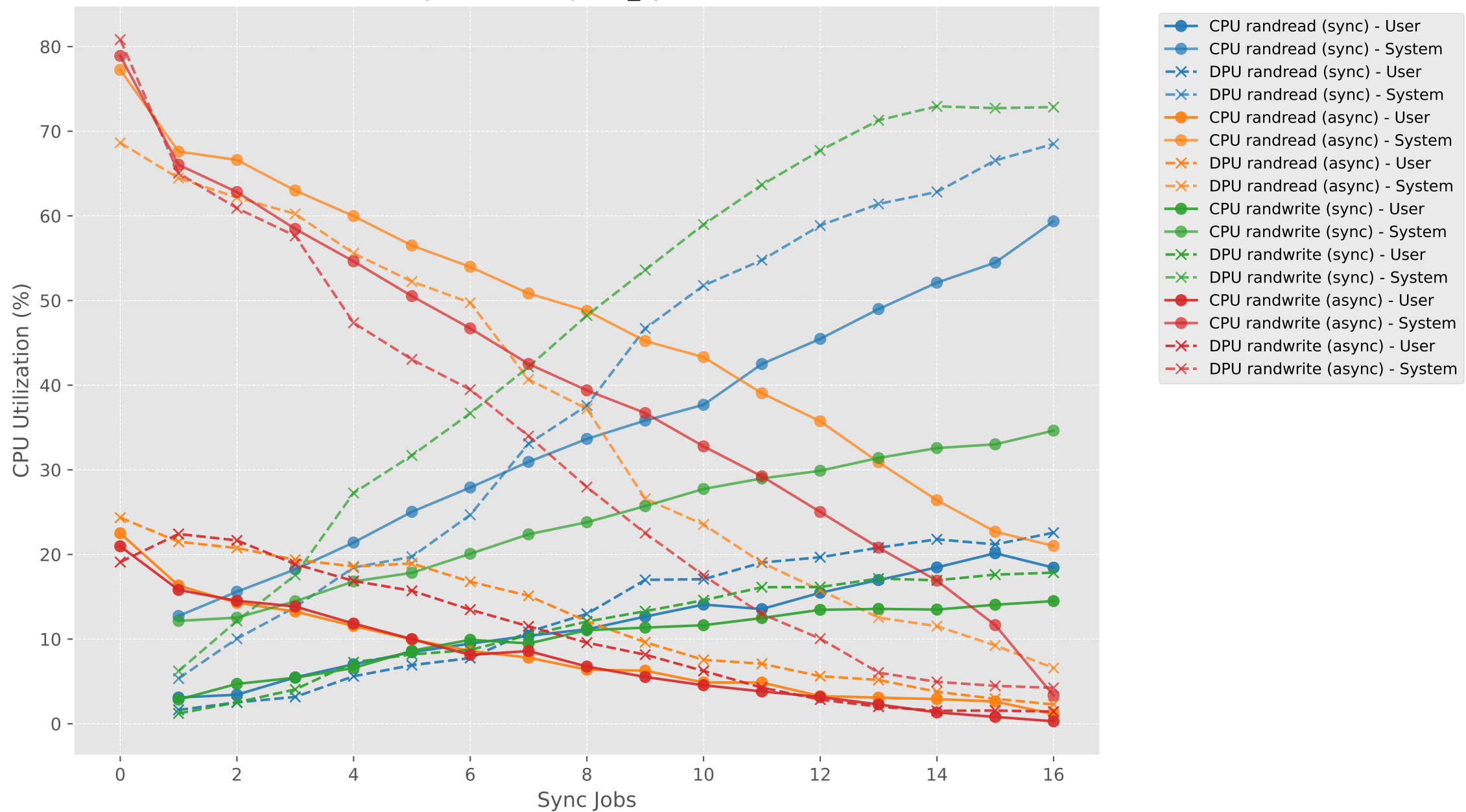
CPU Utilization vs Sync Jobs (async1_syncN) - RAND (CPU vs DPU)
